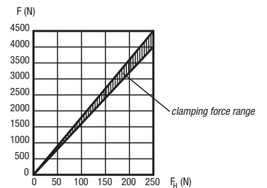
Force diagram
