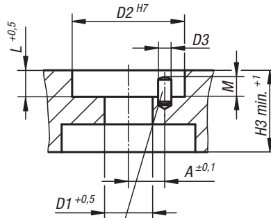
mounting dimensions
