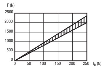
Force diagram
