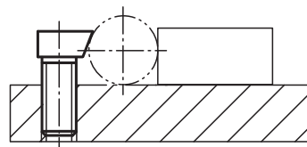
clamping round parts
